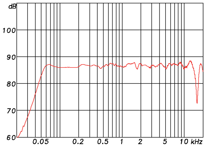
F 6 A hor. directivity plot
