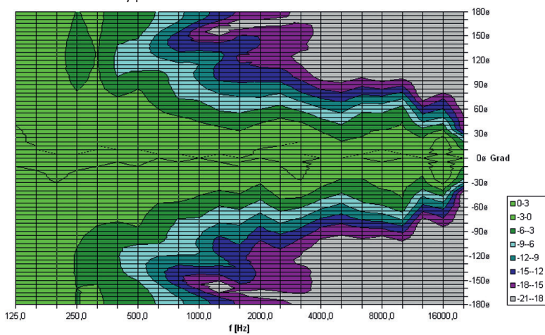
F 6 A vert. directivity plot
