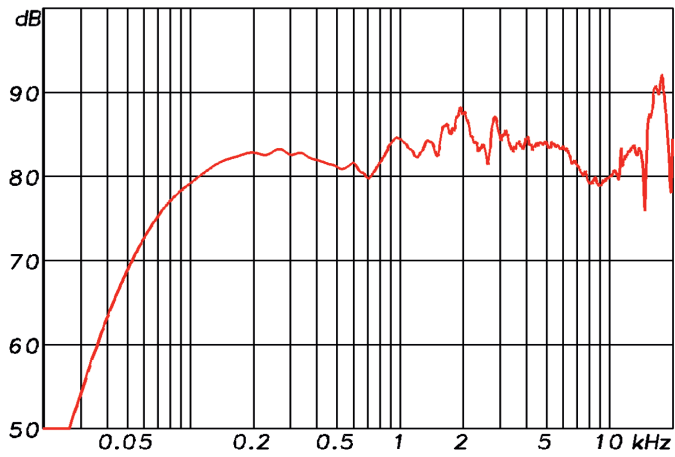
DE 100 Sens. 2.83V/1m: 82.7 dB (100-10k) 77 Hz - 20 kHz (-6 dB) half space
