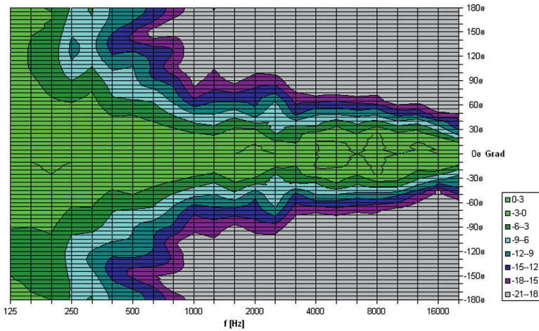
F 12 vert. directivity plot
