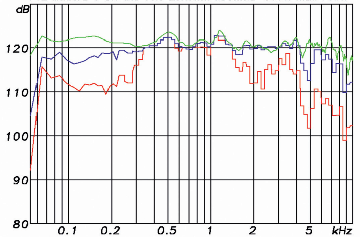
F 12 max. SPL @ 3% and 10% dist. threshold 800 W max. power
