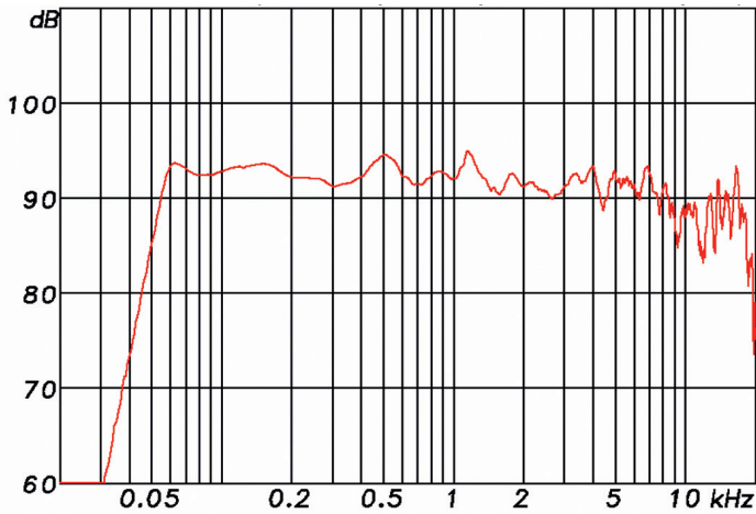
F 12 Sens. 2.83 V/1m: 92 dBb (100-10k) 50 Hz - 18.3 kHz (-6 dB)
