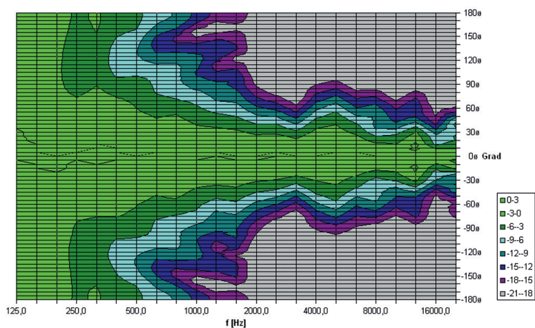
F 8 vert. directivity plot
