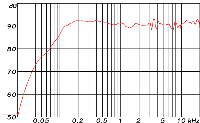
ZL 200 AIArray Sens. @ 2, 83V/1m, d=4m
